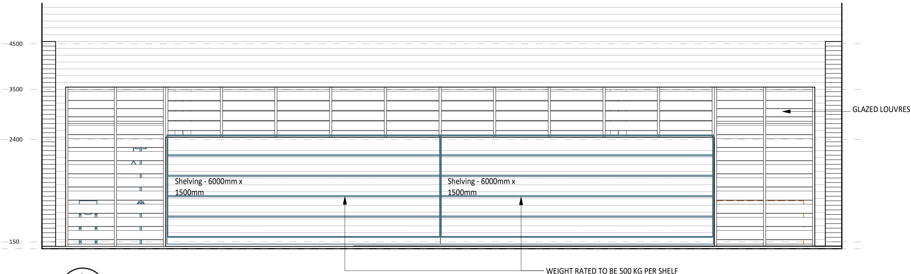
2 ELEVATION DETAIL 1 : 50
